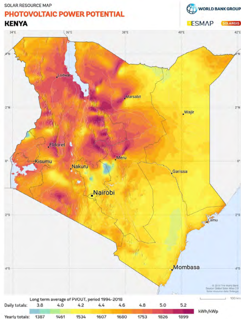
Figure 18: Solar resource map for Kenya
