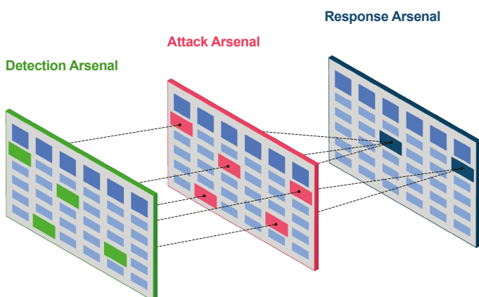
Figure 4: Matrix visualisation of the FIMI Detection, Attack and Response Arsenals inspired by MITRE's offensive and defensive technique relationships (ATT&CK and D3FEND) 50
