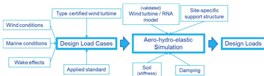
Figure 12 Information required for the load analysis
