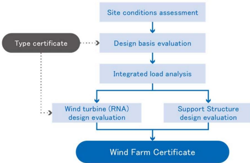
Figure 14 Wind farm certification modules and flow
